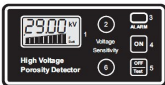
CONTROL LAYOUT
