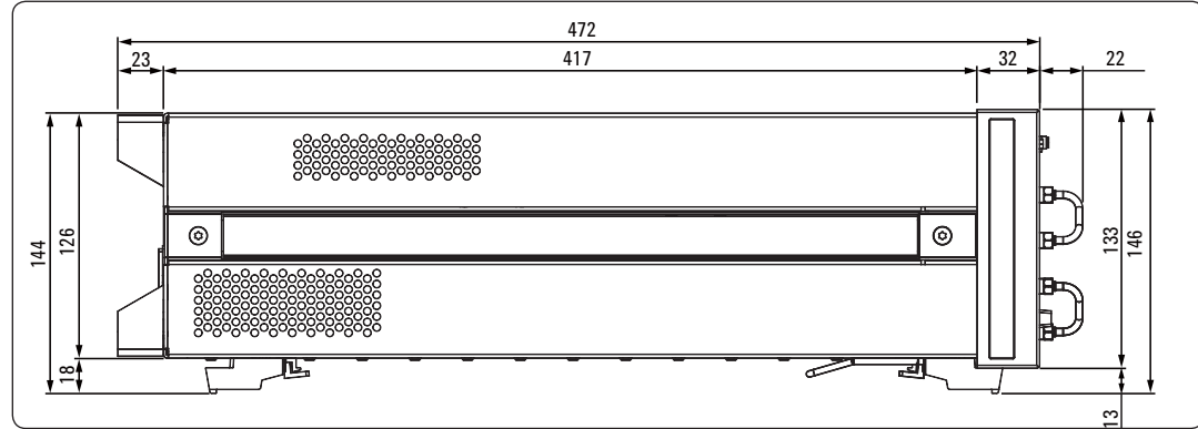
Figure 13. Dimensions (side view, with Option E5092A-020, in millimeters, nominal)
